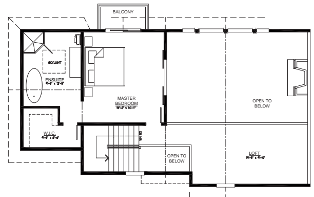
UPPER FLOOR
