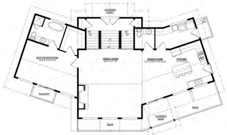
MAIN FLOOR
