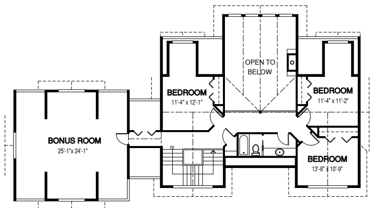
UPPER FLOOR
