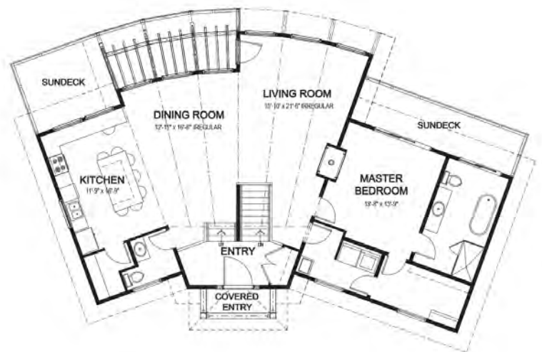
MAIN FLOOR
