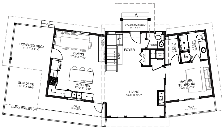
MAIN FLOOR
