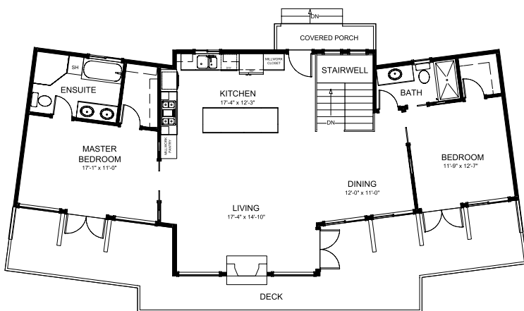
MAIN FLOOR
