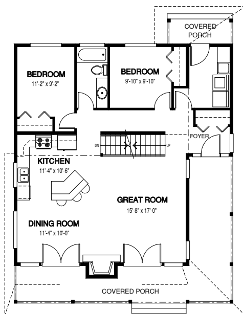
MAIN FLOOR
